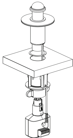
MX395 with A400MB Mute Button Exploded View
