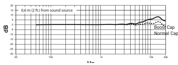
MX150/O Frequency Response
