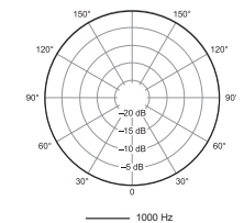
MX150/O Polar Pattern
