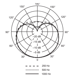
MX150/C Polar Pattern
