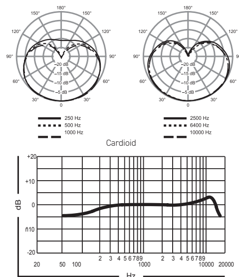
MX415DUAL/C Dual Capsule Gooseneck Microphone
