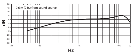
MX150/C Frequency Response
